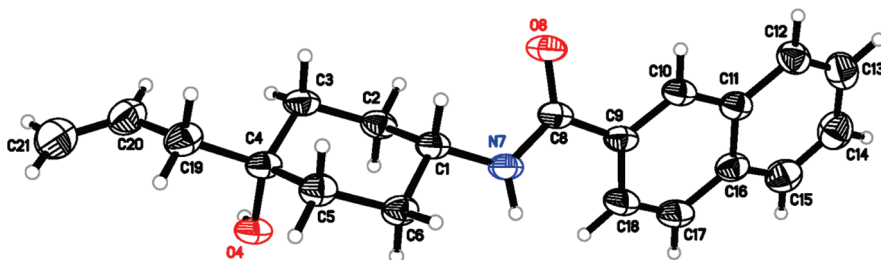
Figure 3. Crystal structure of intermediate 20.
