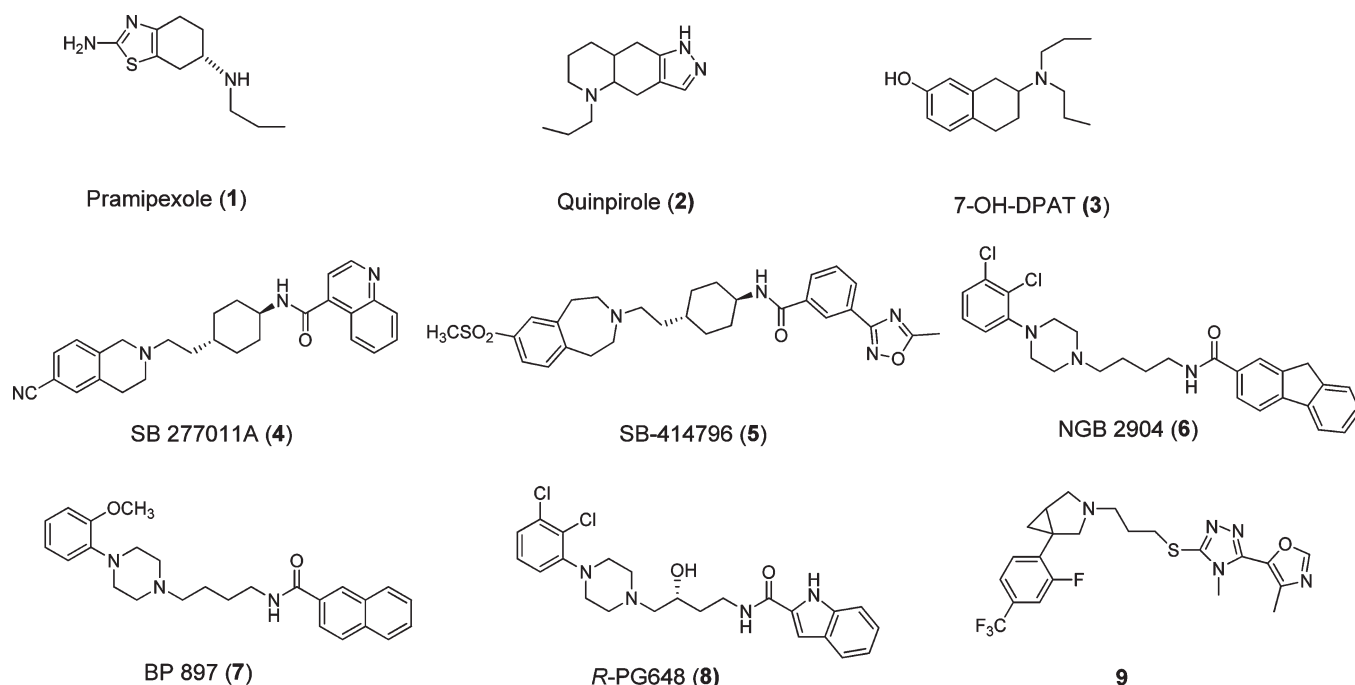
Figure 1. Chemical structures of representative known D3 agonists (1–3) and antagonists (4–9).
